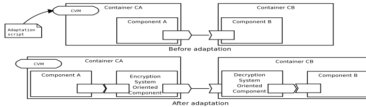
Fig. 4. Integration of the encryption service
